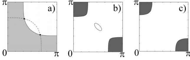
FIG. 1. Evolution of the Fermi surface upon decreasing electron doping x . To distinguish holes from electrons, electrons from the upper band E_{\mathbf{k}}^+ are dark shaded; light shading contains all electrons from both bands. At x=x_c=0.165 , a gap opens at the points where the dispersion crosses its translation by the wave vector (\pi, \pi) [see (a)]. A hole pocket centered at (\pi/2, \pi/2) is present for x_1 < x < x_c (with x_1=0.145 ) as shown in (b) for x=0.15 . For x < x_1 , only electronlike pockets remain as shown in (c) for x=0.12 .
