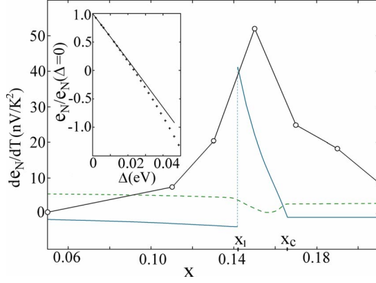
FIG. 2. (Color online) Dependence of the Nernst coefficient on electron doping in the limit T \rightarrow 0 . With decreasing x , the coefficient has an onset near x = x_c , where SDW order sets in. The discontinuity at x = x_1 is due to the opening of hole pockets (blue curve). The magnitude of our estimate of contributions due to energy dependence of the relaxation time has negligible size in the peak region (dashed line), as compared to the experimental values (black curve). Experimental data points from Ref. 5 correspond to the small circles; the line is a guide to the eyes. Inset shows the quantum critical contribution to \vartheta_{yx} , which becomes large already at small gap energies \Delta . Numerical data points in the inset correspond to the crosses, which asymptotically behave as a linear function of gap amplitude, as given by the black line.
