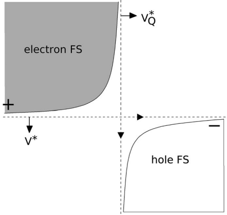
FIG. 3. To leading order in the gap amplitude \Delta , opening of the SDW gap modifies the Fermi surface only near the crossing points in momentum space where \epsilon_{\mathbf{p}} = \epsilon_{\mathbf{p}+\mathbf{Q}} = \mu . As shown in this sketch, a crossing point is coinciding with the crossing of the dashed lines as long as curvature of the Fermi surfaces is neglected near the crossing point. The vertical dashed line is the Fermi line for the normal state which is parallel to the vector (0, \pi) . The horizontal dashed line is the normal-state Fermi line shifted by \mathbf{Q} = (\pi, \pi) , thus directing parallel to (\pi, 0) . The reconstructed Fermi surface contains electron pockets, denoted by +, and hole pockets, denoted by -.
